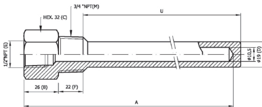
Standard BETA Thermowell
